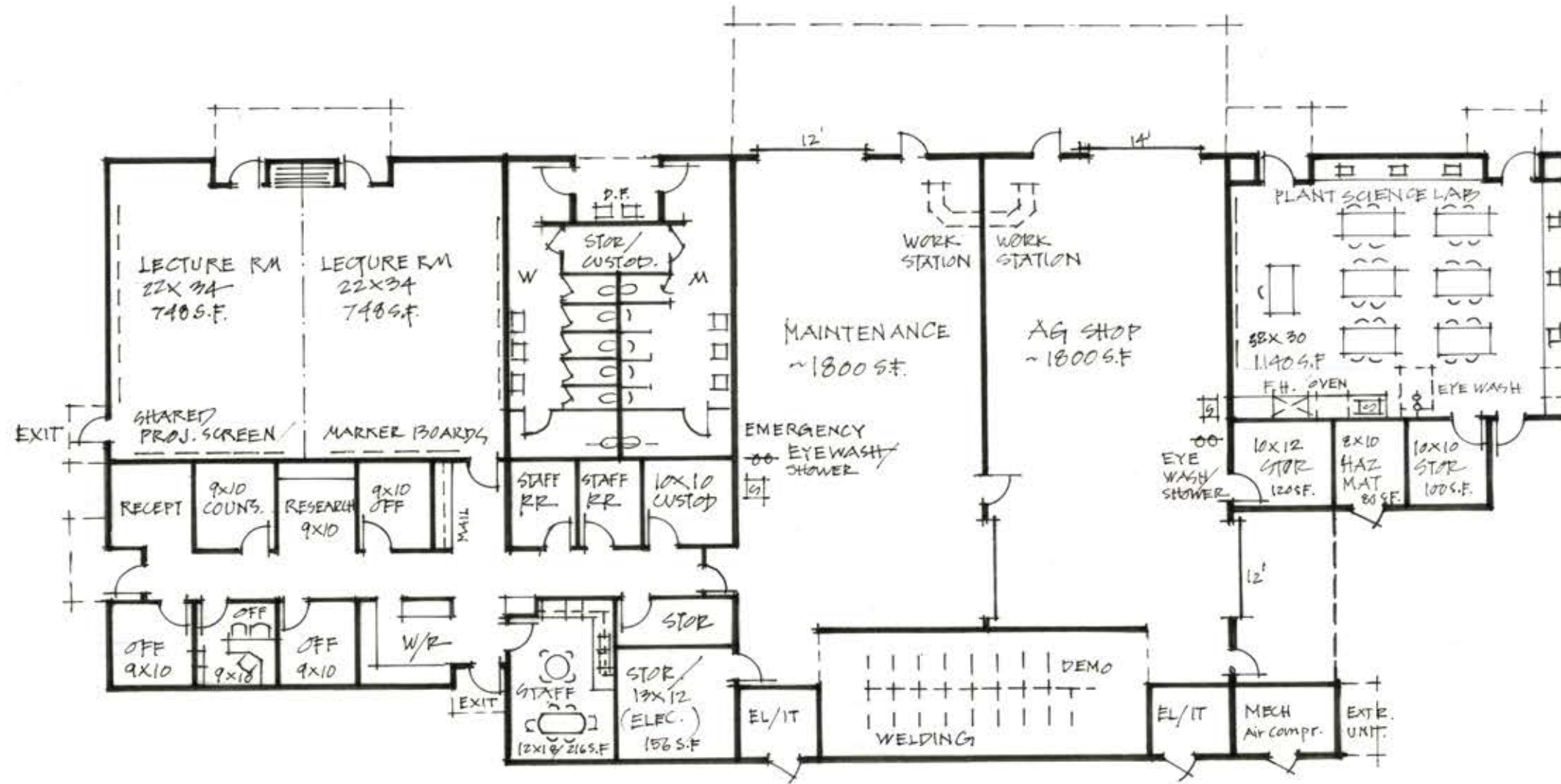
Revised FLOOR PLAN 1/16" = 1'-0"
